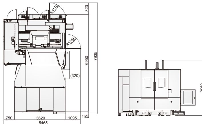
HK-LH-800(A) / 1000(A)
